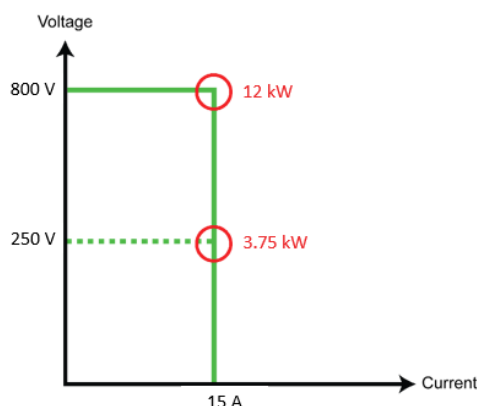
Figure 2. Rectangular output characteristic of a conventional 12 kW supply
