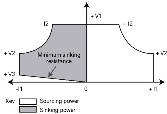
Figure 7. RP5900 output characteristic
