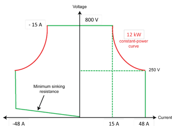
Figure 1. Autoranging output characteristic of the 12 kW RP5946A
